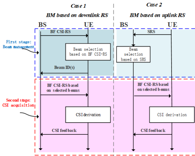
FIGURE 2. Two stage CSI framework.
