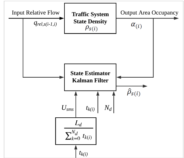
FIGURE 1. Block diagram of the proposed work.
