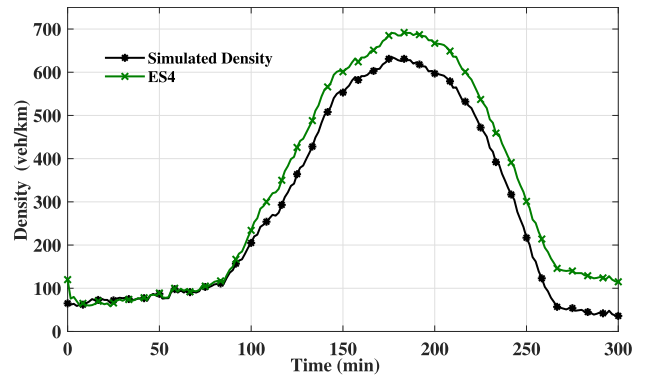
FIGURE 6. Corroboration of ES4 scheme for scenario 1 (transition).
