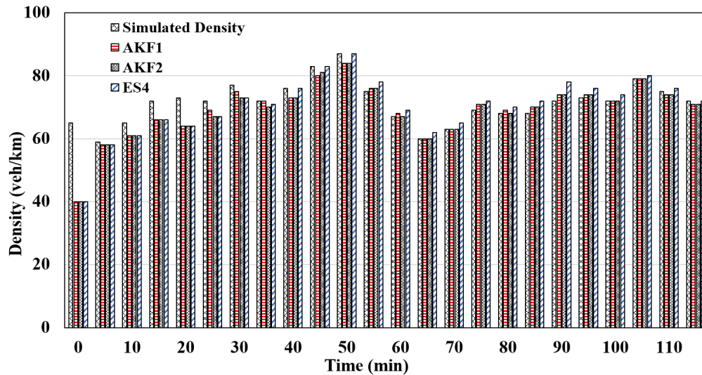
FIGURE 9. Performance comparisons under scenario 2 (light traffic).
