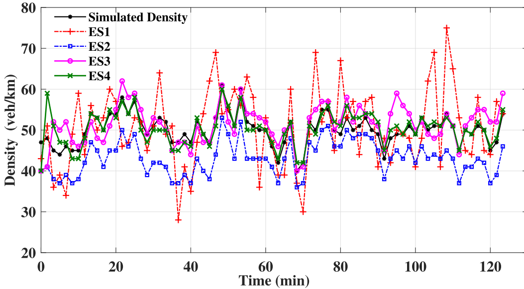
FIGURE 4. Corroboration of the all four density estimation schemes.
