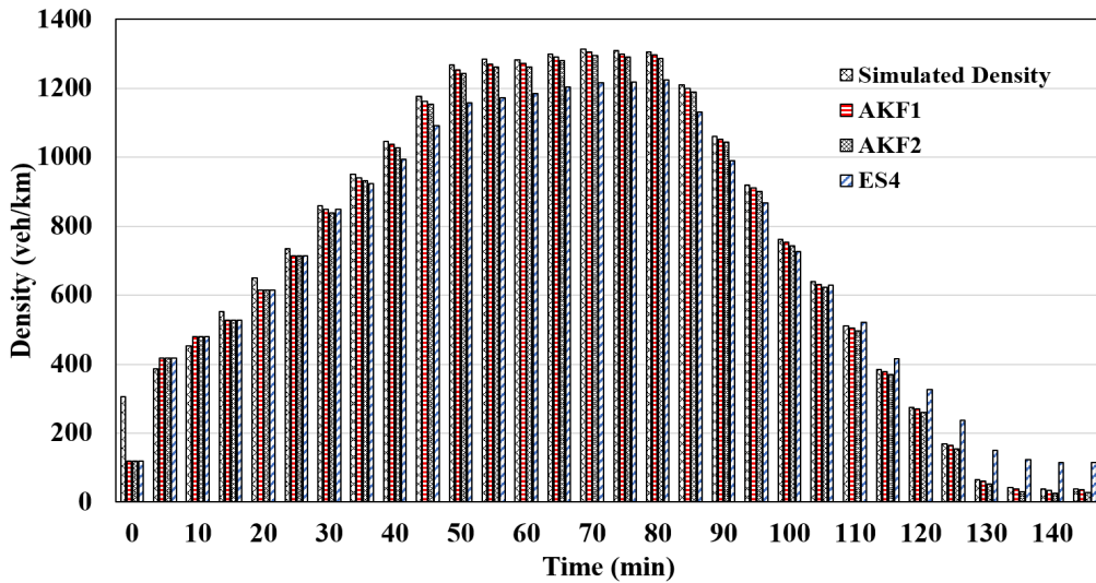
FIGURE 10. Performance comparisons under scenario 3 (jam density).
