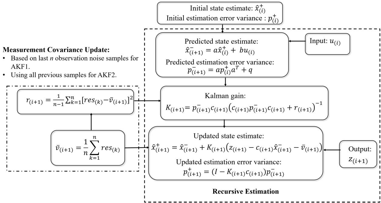
FIGURE 7. Algorithm for adaptive Kalman filter schemes.
