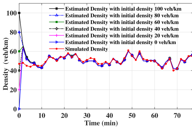
FIGURE 5. Convergence for different values of initial density.
