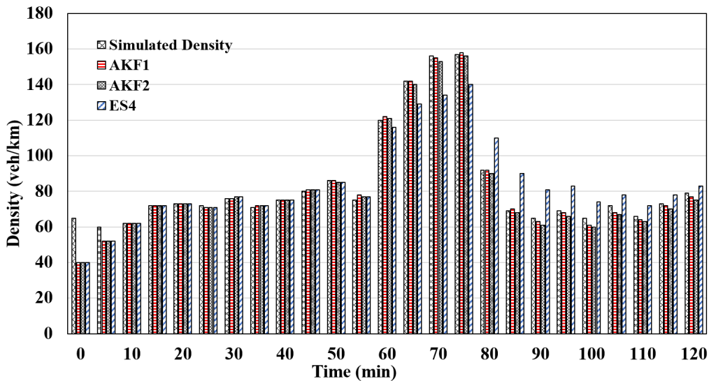
FIGURE 11. Performance comparisons under scenario 4 (incident).
