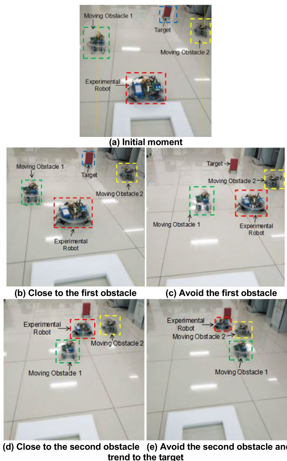
FIGURE 15. Experimental process to avoid movement obstacles.
