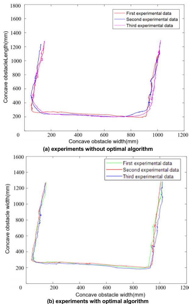
FIGURE 12. Path planning for the spherical mobile robot in the concave environment.
