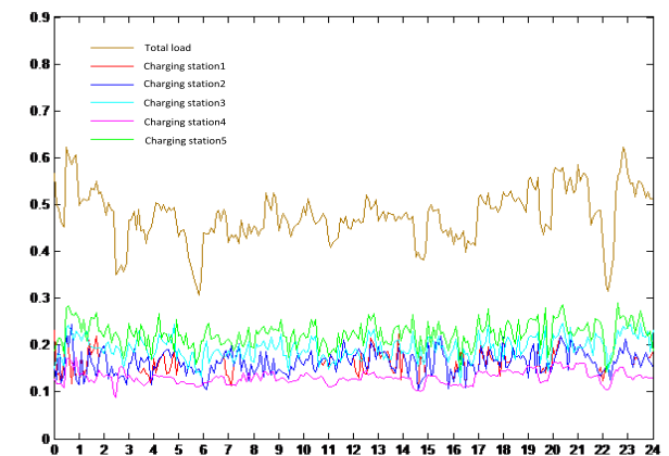
FIGURE 7. Load curve of each charging station.
