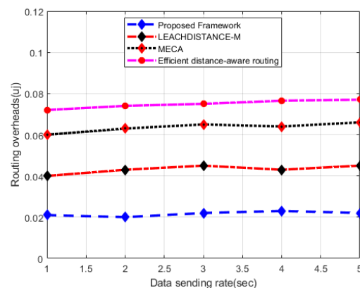
FIGURE 12. The impact of a data sending rate on routing overheads.
