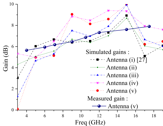
FIGURE 7. Measured and simulated gains of the proposed antennas.
