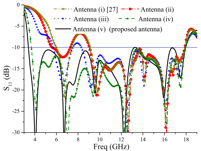
FIGURE 2. (a) Evolution of the proposed antenna, (i) the design of [27], (ii), (iii), (iv), (v) steps of design optimization. (b) simulated S_{11} of the five designs shown in (a).
