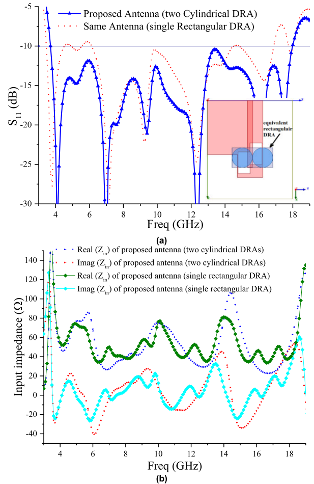
FIGURE 5. (a) Simulated S_{11} of 2-cylindrical DRA compared to a single rectangular DRA with the same overall dimensions, (b) Simulated input impedance of 2-cylindrical DRA compared to a single rectangular DRA.
