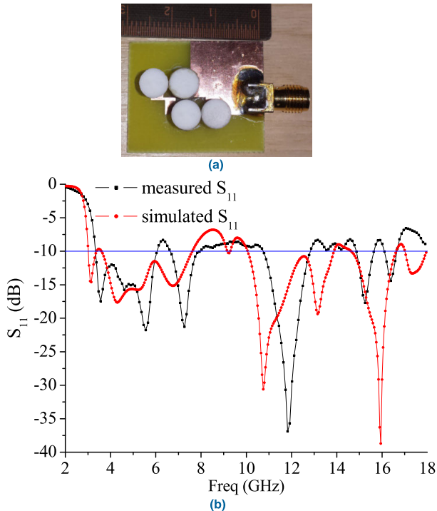
FIGURE 13. (a) Proposed antenna with four DRs (3 rd configuration) (b) Simulated and measured S_{11} of 4-DR antenna.
