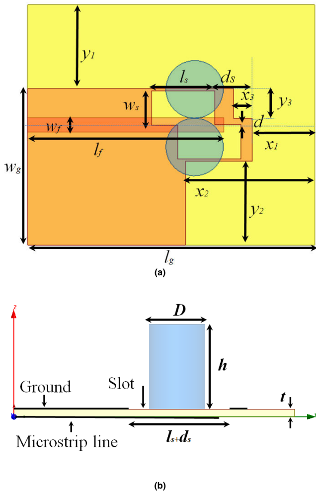
FIGURE 1. Design parameters of two aperture-coupled DRAs with non-uniform defected ground plane, (a) top view and (b) side view.
