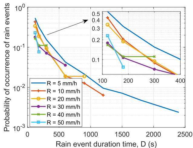
FIGURE 5. Probability of occurrence of rain events.
