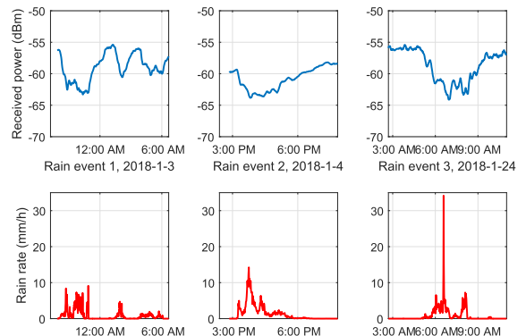
FIGURE 12. Measured co-polarisation attenuation for different rain and snow events at 77.52 GHz.
