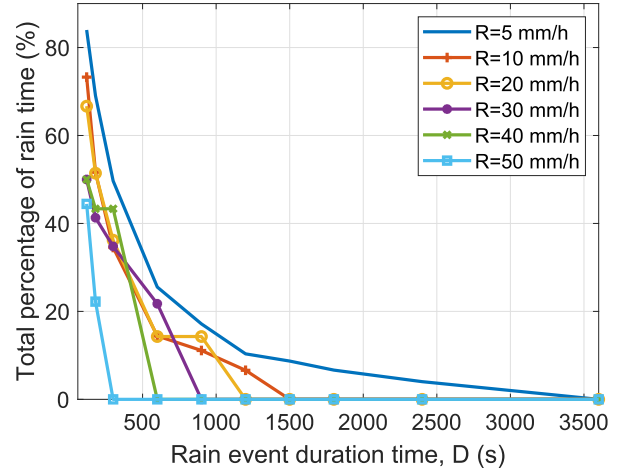
FIGURE 6. Total percentage of rain time.
