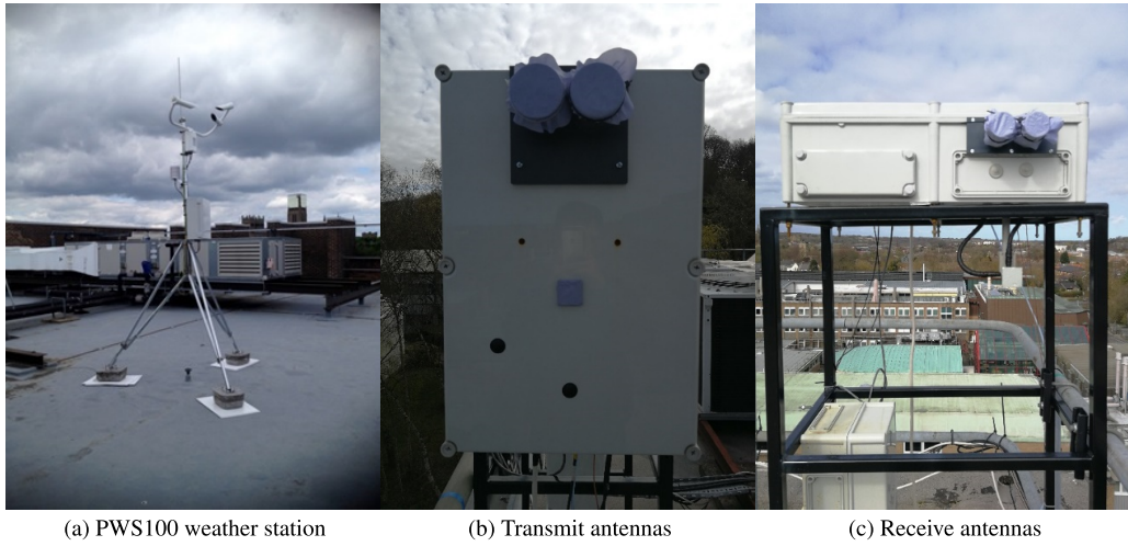
FIGURE 1. Transmit and receive antennas with coverage of radomes.
