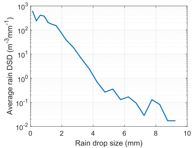
FIGURE 7. Average rain DSD over all rain bins.
