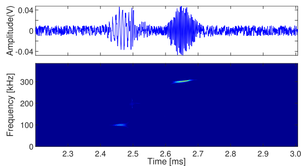
FIGURE 12. The wavepacket W_5 and its reassigned distribution.
