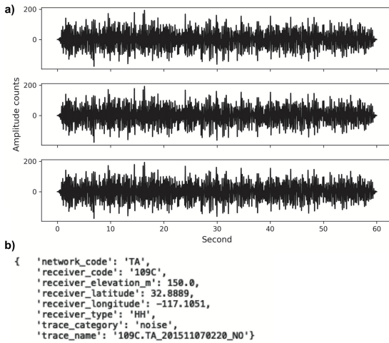
FIGURE 7. Example of noise data. a) time-series ground motions for east-west, north-south, and vertical directions respectively. b) header information (labels) associated with the seismogram.
