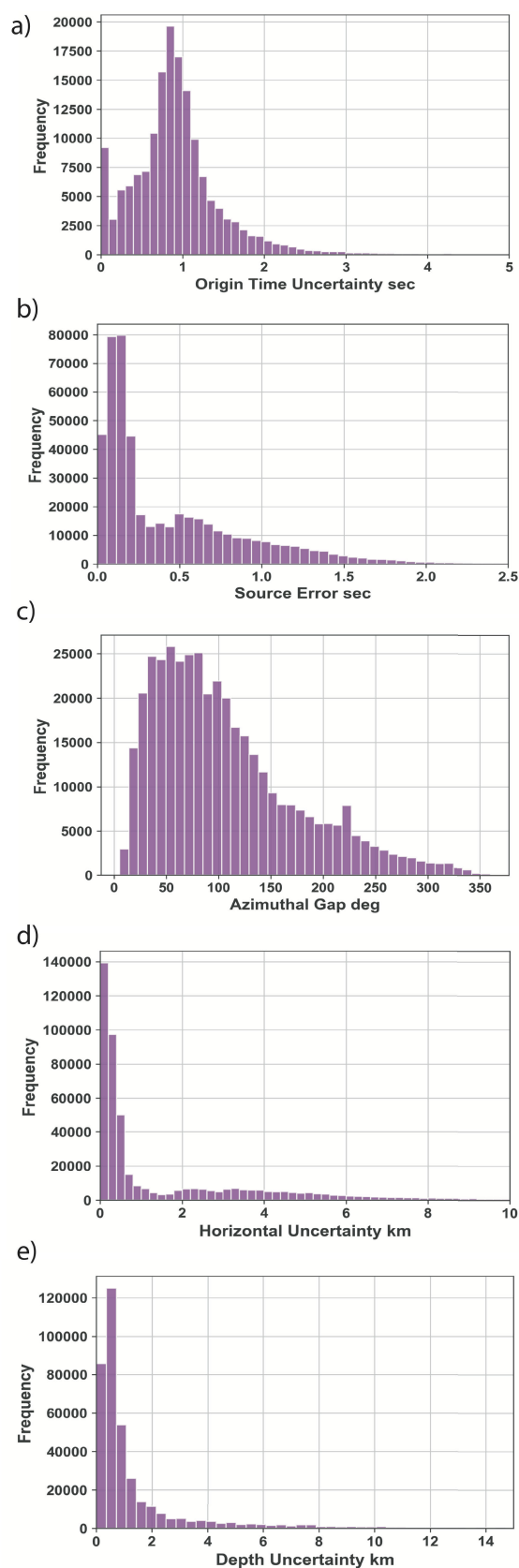
FIGURE 18. Uncertainties in the earthquake characterization.
