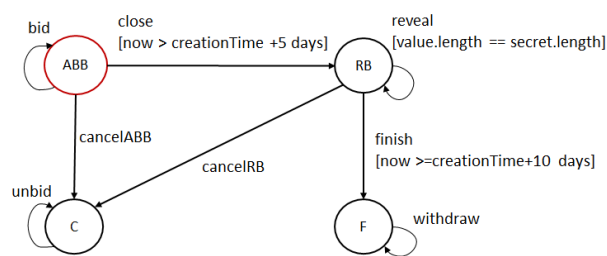
FIGURE 11. An example of FSM for blind auctions from [46].
