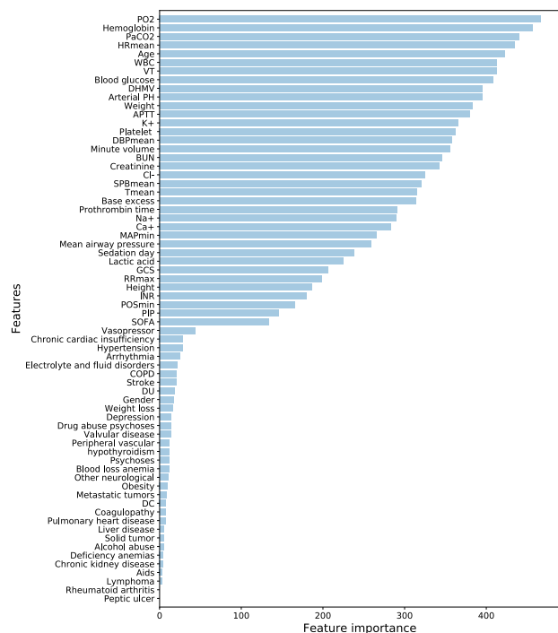
FIGURE 7. The feature importance ranking of XGboost (with 68 features).
