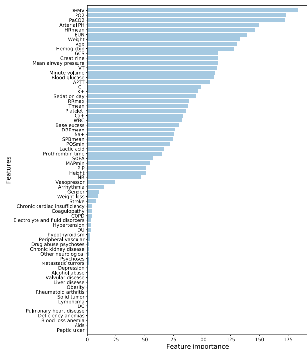
FIGURE 6. The feature importance ranking of LightGBM (with 68 features).
