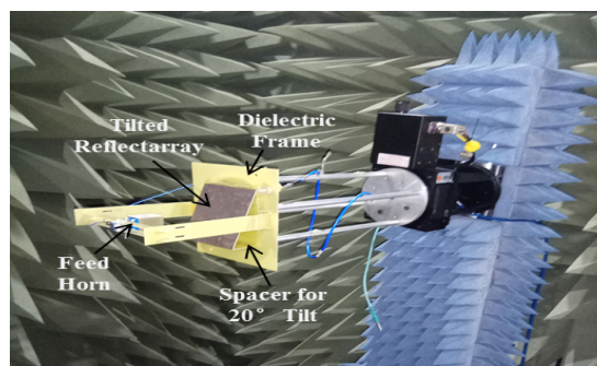
FIGURE 4. Radiation pattern measurement setup in the anechoic chamber.
