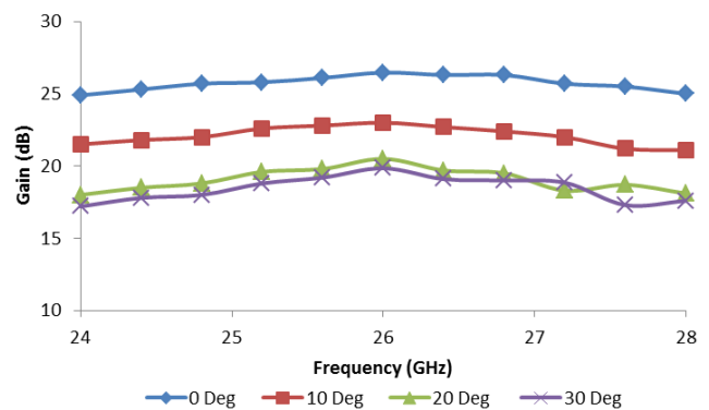
FIGURE 10. Measured gain vs frequency plots for different tilt angles.
