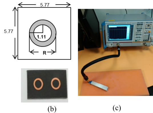
FIGURE 1. Proposed reflectarray unit cell (a) Design configuration (b) Fabricated two patch element unit cell (c) Scattering parameter measurement setup.
