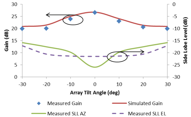
FIGURE 9. Gain and side lobe levels for different reflectarray tilt angles.
