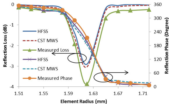
FIGURE 2. Measured and simulated scattering parameters of reflectarray unit cells.
