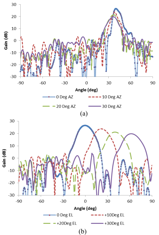
FIGURE 7. Measured radiation patterns for scanned beam reflectarray at different tilt angles (a) Azimuth plane (b) Elevation plane.
