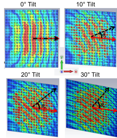
FIGURE 6. Phase of the surface current distribution of different tilt angles.
