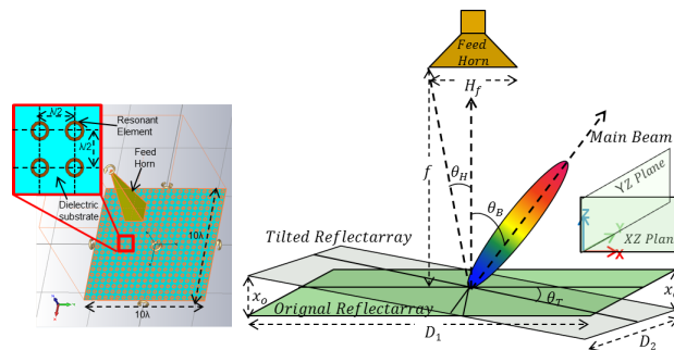
FIGURE 3. Complete assembly of the simulated reflectarray and its schematic diagram.
