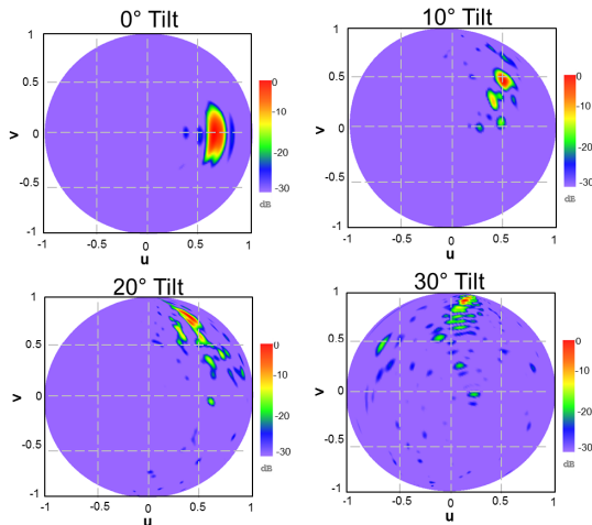
FIGURE 8. Measured 3D Co-polar components in UV plane for different tilt angles of reflectarray.
