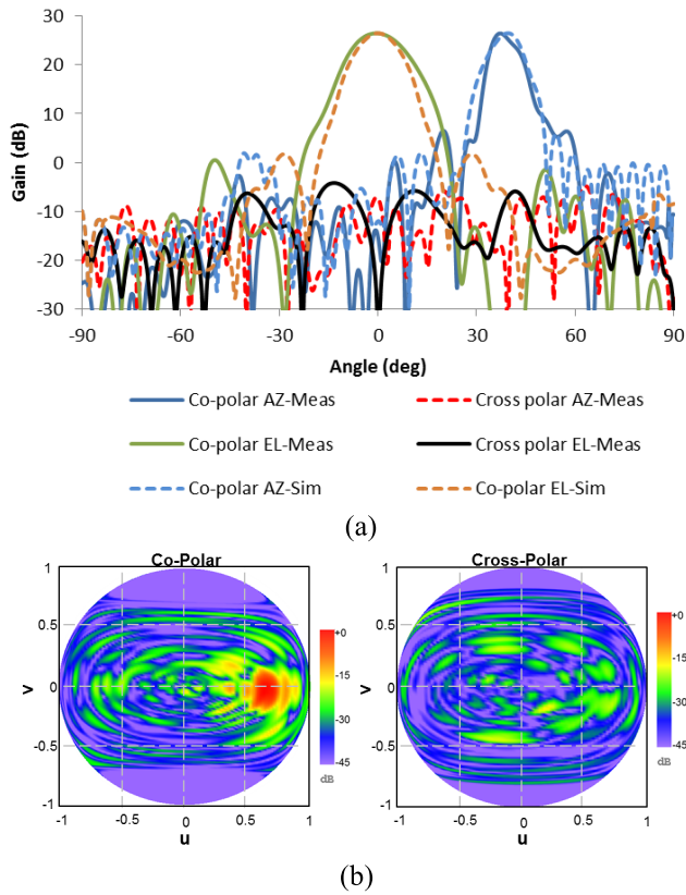
FIGURE 5. Radiation pattern results for fixed beam reflectarray at 26 GHz (a) Measured and simulated azimuth and elevation planes in cartesian coordinates (b) Three dimensional measured results in UV plane.
