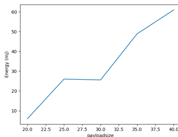
FIGURE 11. Effect of No of end devices on energy (in millijoules) having ADR Enabled.
