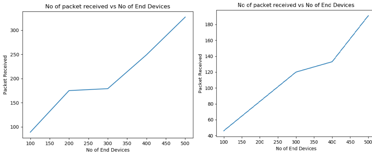
FIGURE 6. Average number of packets received w.r.t No. of end devices with ADR enabled. (a) d=500m (b) d=1000m.
