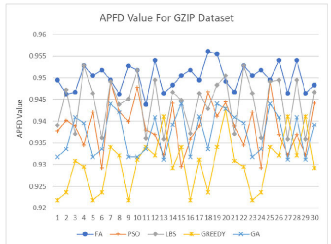
FIGURE 14. APFD graph for GZIP benchmark program.
