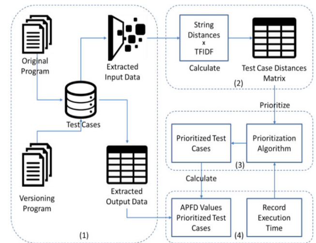
FIGURE 6. Overview of experiment flow.
