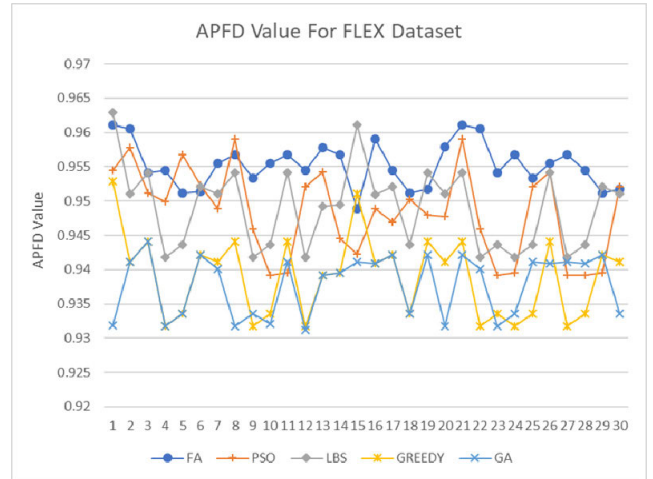
FIGURE 13. APFD graph for FLEX benchmark program.
