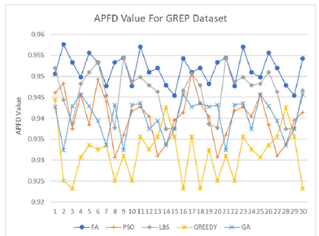
FIGURE 15. APFD Graph for GREP benchmark program.
