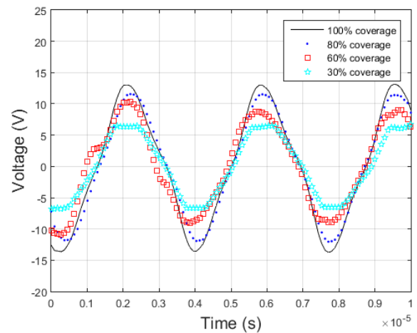
FIGURE 13. Voltage measured on the receiver after a change in misalignment between the coils.
