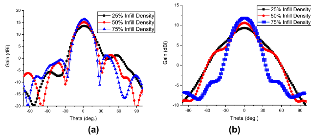
FIGURE 6. Radiation pattern of ILAs at 28 GHz for different infill densities of dielectric lens materials (a). SIW (b). MPA.
