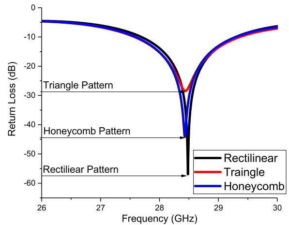
FIGURE 4. Impact of different infill pattern of dielectric lens on the reflection coefficient.
