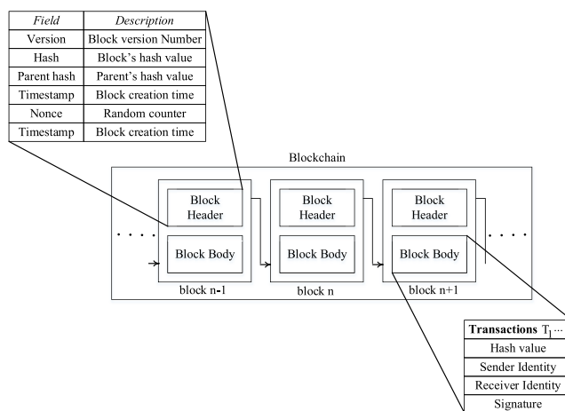
FIGURE 3. Blockchain structure.
