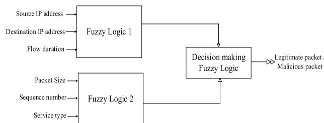
FIGURE 4. Multi-Fuzzy model.
