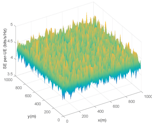
FIGURE 3. SE per-UE of the CF massive MIMO downlink within a square area of 1 \times 1 \text{ km}^2 ( M = 100, K = 10 ).
