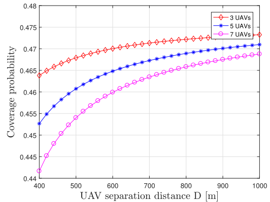
FIGURE 8. Boundary user coverage probability in the primary USC for the severe interference generated from secondary UAVs for different number of UAVs in urban environment.
