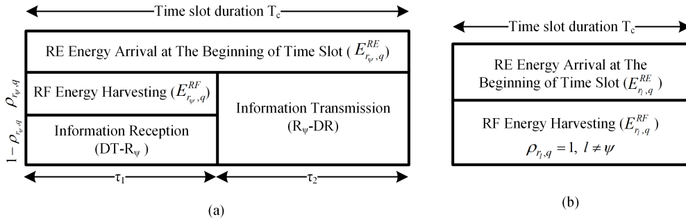
FIGURE 2. Block diagram of RE and RF EH model during time slot q for (a) selected relay (b) non-selected relay.
