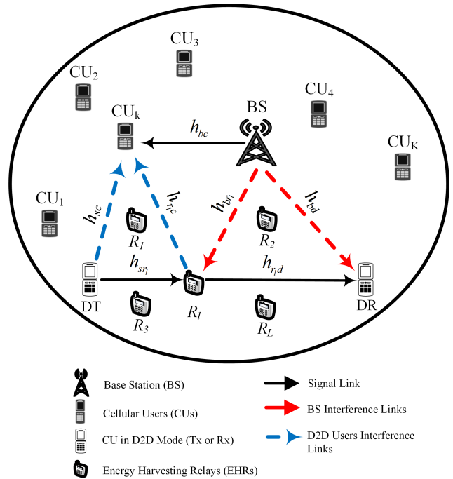
FIGURE 1. System model of the relay-aided D2D communication underlying conventional DL cellular network.
