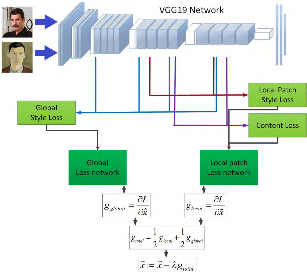
FIGURE 3. Our neural style transfer framework.
