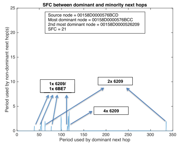
FIGURE 8. Switching Frequency Count between source router 6BCD and its dominant next hop router 6BCC.
