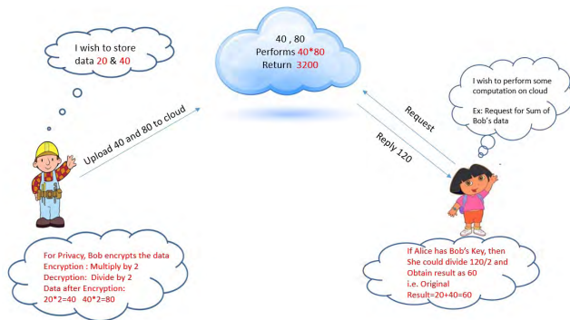
FIGURE 9. Example of homomorphic encryption.
