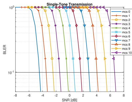
FIGURE 15. Simulation results for GS-T with different MCS levels.
