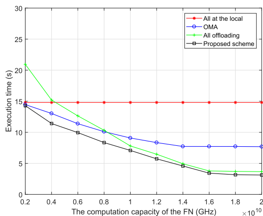
FIGURE 16. Average delay versus the computation capacity of the FN.
