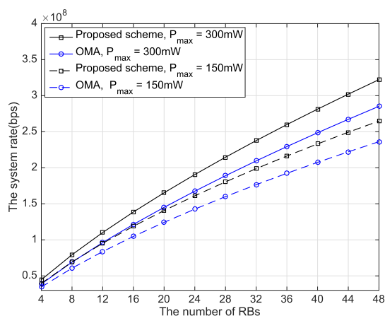
FIGURE 8. System rate versus the number of RBs.
