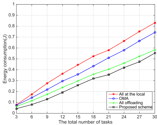
FIGURE 12. Energy consumption versus the number of tasks.
