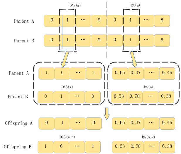
FIGURE 4. The process of crossover operation.
