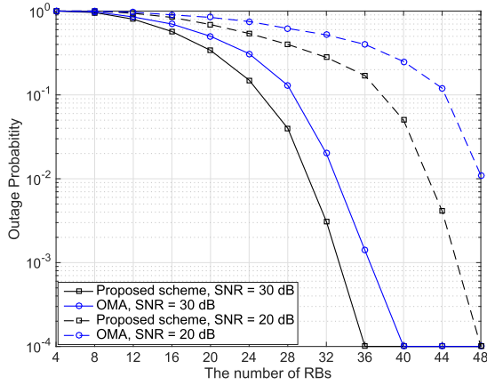
FIGURE 11. Outage probability versus the number of RBs.
