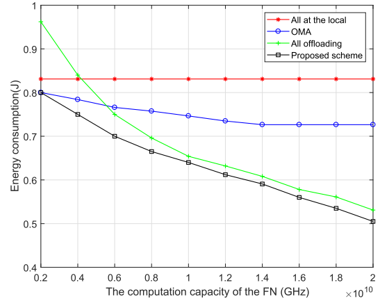
FIGURE 13. Energy consumption versus the computation capacity of the FN.
