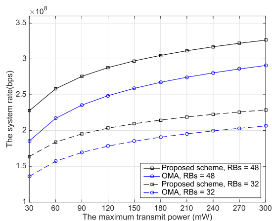
FIGURE 9. System rate versus the maximum of transmit power.
