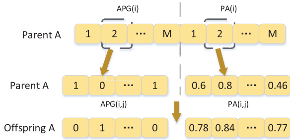
FIGURE 5. The process of mutation.
