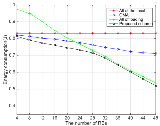
FIGURE 14. Energy consumption versus the number of RBs.
