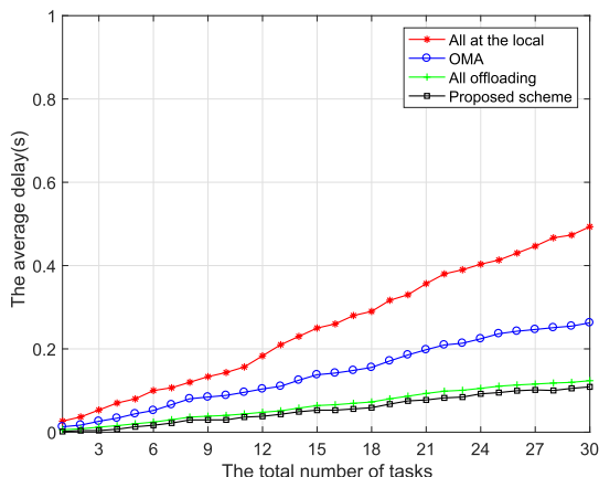
FIGURE 15. Average delay versus the number of tasks.
