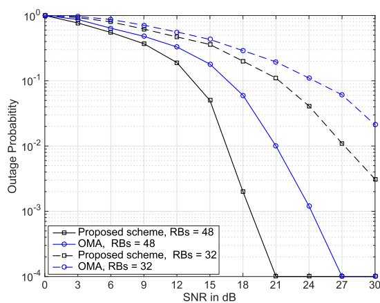
FIGURE 10. Outage probability versus SNR.
