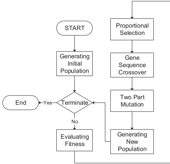
FIGURE 3. Flow diagram of IGA.
