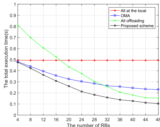
FIGURE 17. Average delay versus the number of RBs.
