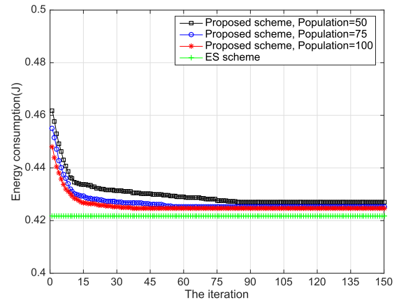
FIGURE 6. Energy consumption versus the iterations.
