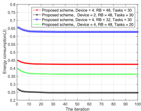
FIGURE 7. Convergence performance with devices/tasks/RBs.
