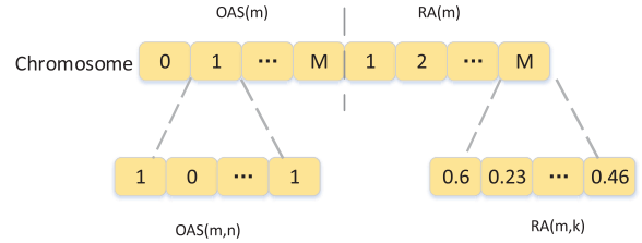
FIGURE 2. The structure of the chromosome.
