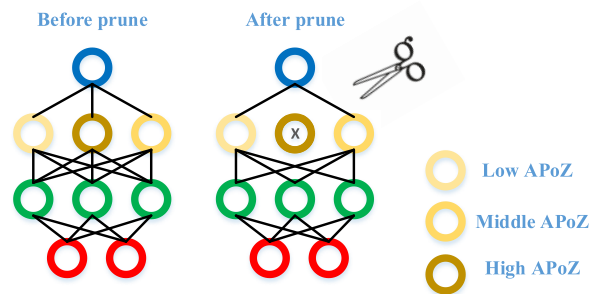
FIGURE 4. Convolution filter level pruning base on APoZ.
