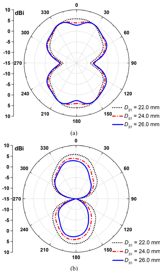
FIGURE 9. Simulated radiating patterns of the proposed antenna respect to different D_{S1} @ 3.15 GHz. (a) E -plane; (b) H -plane. The other parameters are: L = 82.0 mm, W = 4.0 mm, L_G = 140.0 mm, W_G = 90.0 mm, L_{S1} = 16.4 mm, L_{S2} = 15.5 mm, and D_{S2} = 18.0 mm.
