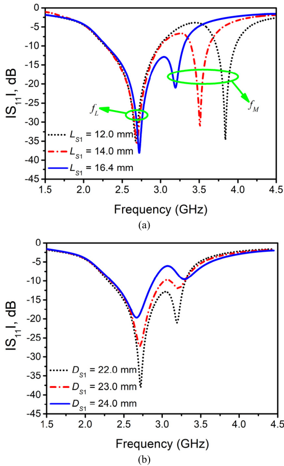
FIGURE 3. Reflection coefficient S_{11} of a dual-band slotline antenna with respect to different (a) L_{S1} ( D_{S1} = 22.0 mm); and (b) D_{S1} ( L_{S1} = 16.4 mm). The other parameters are: L = 82.0 mm, W = 4.0 mm, L_{S2} = 0 , L_G = 140.0 mm, and W_G = 90.0 mm.
