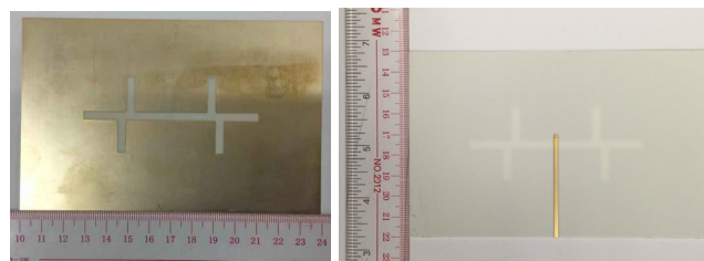
FIGURE 11. Photograph of the prototype antenna fed by a 50- \Omega short-ended microstrip line.
