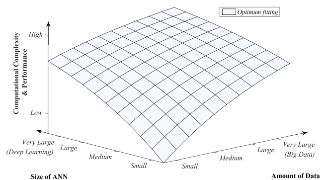
FIGURE 2. Performance of Artificial Neural Networks as a function of Big-Data availability and learning level, i.e., computational complexity.
