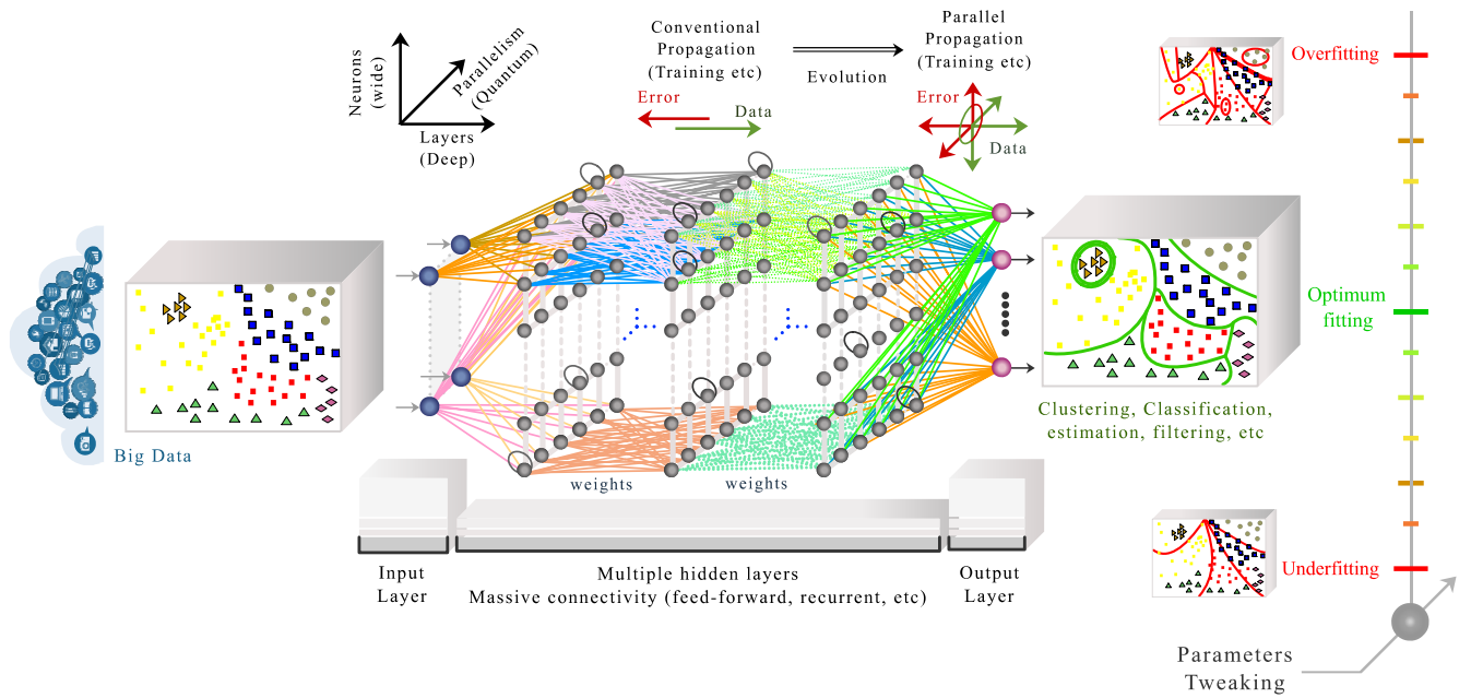
FIGURE 3. An example of a complex artificial neural network structure. Evolution from sequential to parallel data processing and optimum balance between overfitting and underfitting is illustrated.
