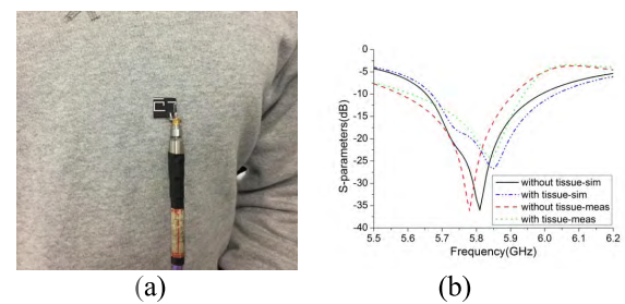
FIGURE 6. Antenna measurement and results. (a) Measure on author's chest, (b) simulated and measured impedance bandwidth.
