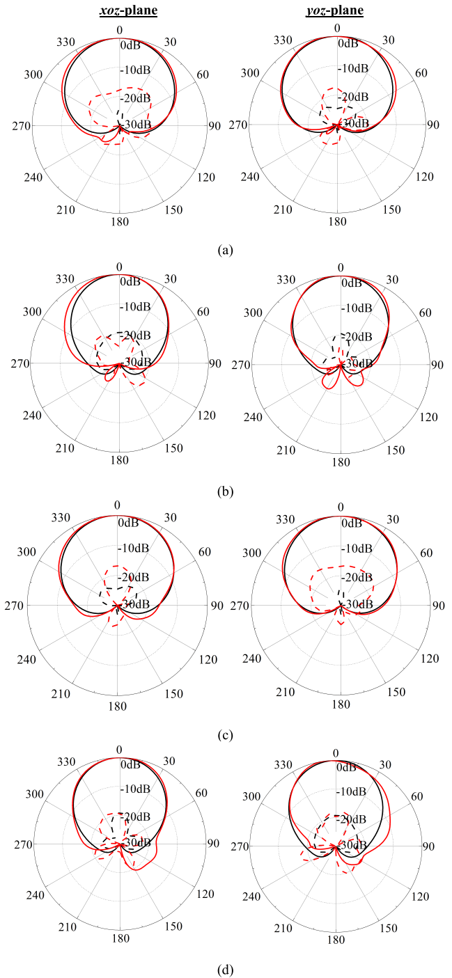
FIGURE 8. Simulated and measured radiation patterns in two states: (a) 1.84 GHz in LHCP; (b) 2.4 GHz in LHCP; (c) 1.84 GHz in RHCP; (d) 2.4 GHz in RHCP.
