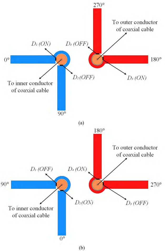
FIGURE 3. RHCP and LHCP states of the crossed dipoles: (a) RHCP state; (b) LHCP state. (Red and blue lines represent the two crossed dipoles, respectively.)
