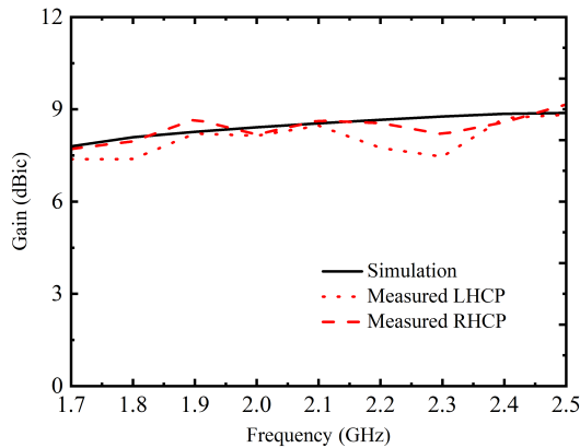
FIGURE 7. Simulated and measured broadside gains.
