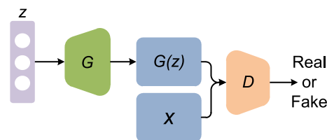
FIGURE 1. The architecture of generative adversarial networks.
