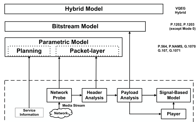
FIGURE 3. QoE model classification for streaming applications (adapted based on input from [30]).
