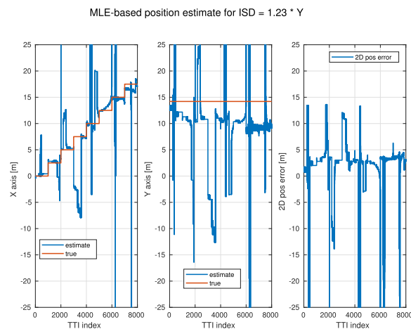
FIGURE 9. Position estimate using MLE-based AoA for the case of ISD = 1.23 * Y = 17.5\text{ m} .
