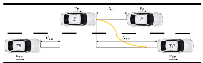
FIGURE 1. Autonomous vehicle lane change model. G_{TR} , G_{TP} , G_P - the longitudinal gap distance between E and TR , TP , P ; v_E , v_{TR} , v_{TP} , v_P - the longitudinal speed of E , TR , TP , and P .
