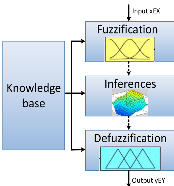
FIGURE 3. Fuzzy system architecture.
