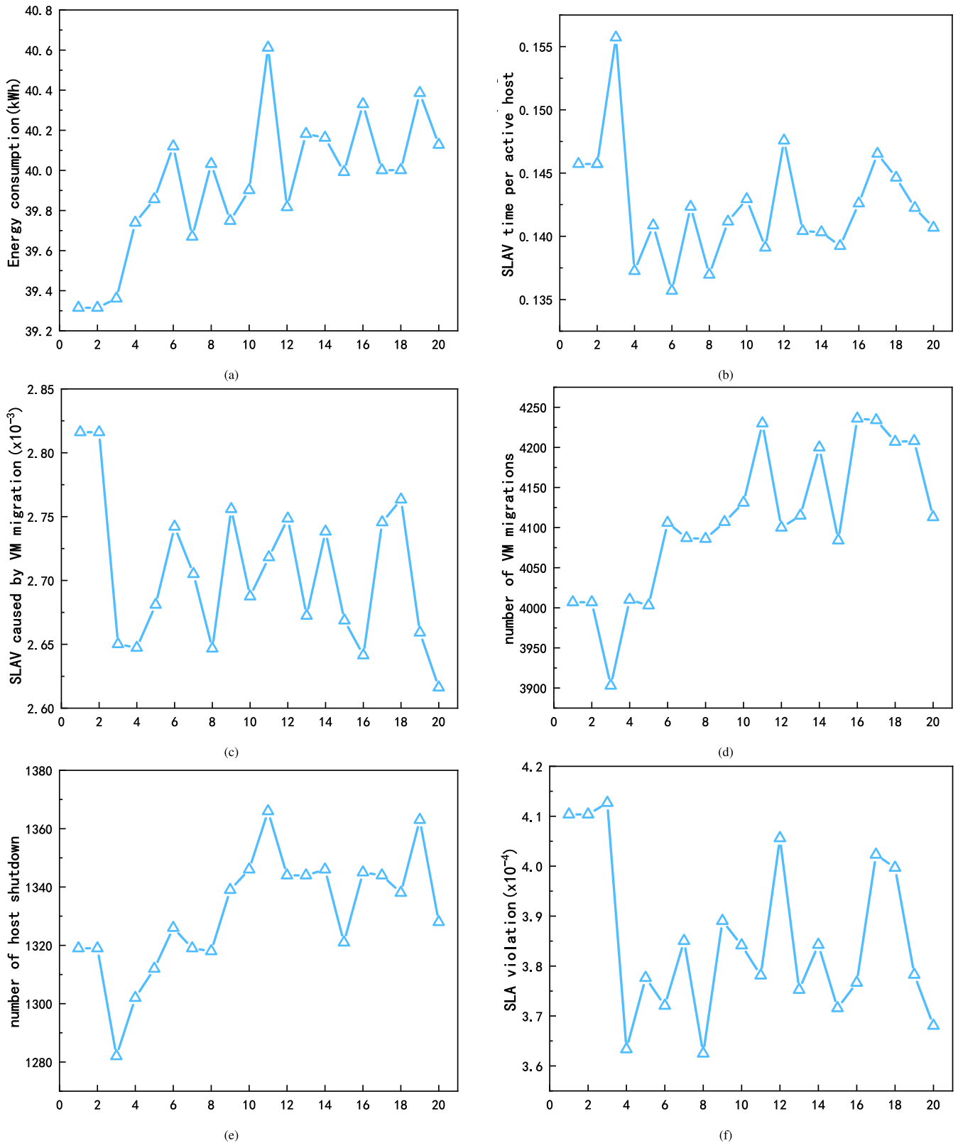
FIGURE 3. The impact of \lambda parameters on WPA performance (illustrated by the case of random workload). (a) The EC metric. (b) The SLATPAH metric. (c) The SLAPDM metric. (d) The NVMM metric. (e) The NHS metric. (f) The SLAV metric.
