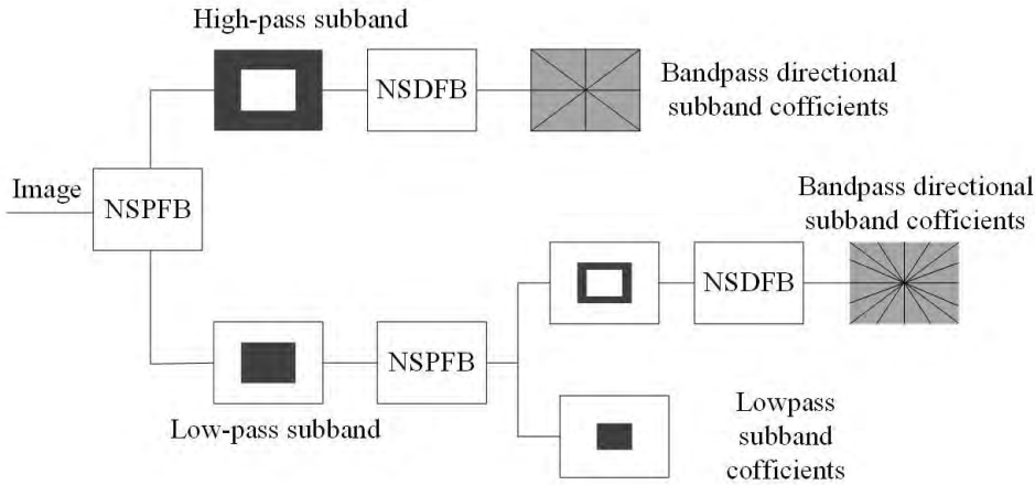
FIGURE 1. Nonsubsampled contourlet transform.
