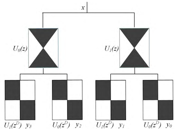
FIGURE 3. Non-subsampled directional filter bank.
