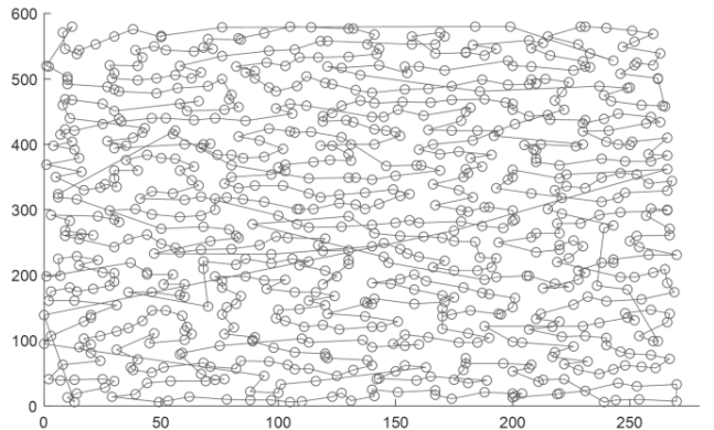
FIGURE 9. The optimal path of rat783(9229).
