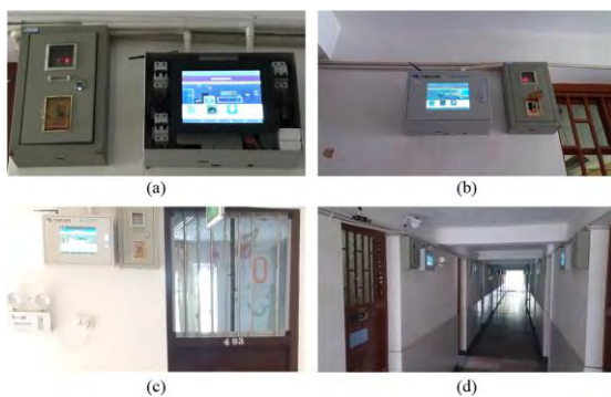
FIGURE 20. Illustration of the field installation of the developed energy internet AE, where (a), (b) and (c) demonstrate that the developed household concentrators have been installed at different locations and are connected in series between the power bus of grid and the original distribution box, and (d) shows that multiple energy internet AE household concentrators have been installed in the selected student dormitory building.
