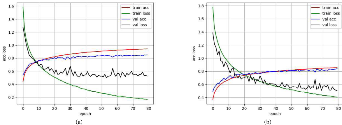
FIGURE 5. The loss and accuracy of the QCNN and the attention based QCNN during the training and testing. (a) QCNN. (b) Attention_based QCNN.
