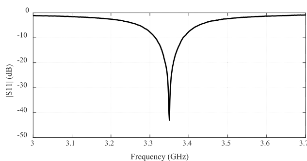
FIGURE 13. Measured reflection coefficient at input ports.
