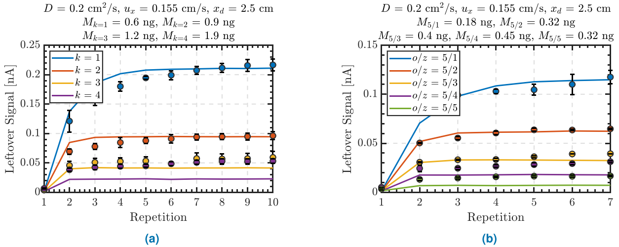
FIGURE 9. (a) Experimental results of the leftover chemicals from k experiment along with theoretical comparison (b) Experimental results of the o/z bit transmission with comparison to the theoretical model.
