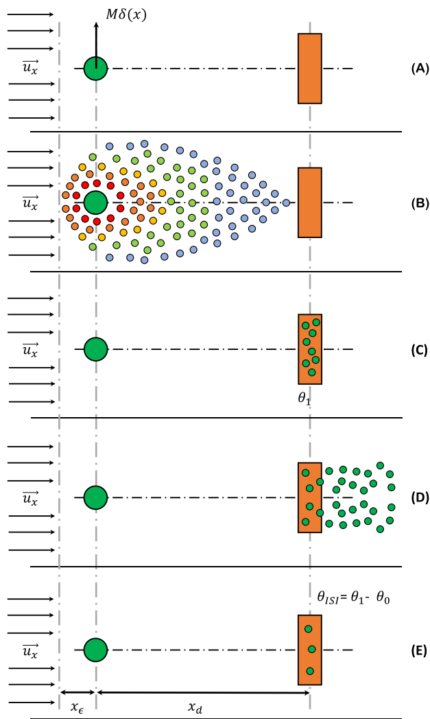
FIGURE 3. A diagram of the model used in the study (A) At t = 0 s mass is injected into the environment. This is defined by the initial boundary condition C(x_0, t_0) = M\delta(x) (B) As the transmission evolves, the particles start propagating via advection and diffusion (C) When the specified period is passed the transmitter stops releasing particles and transmits only advective flow (D) The flow then forces the particles to be transferred from the detector to the outside environment (E) After a finite amount has passed the particles are removed from the detector and transferred to the outside environment. However, some particles are left in the detector, which can cause inter-symbol interference for future transmissions ( \theta_{ISI} ).
