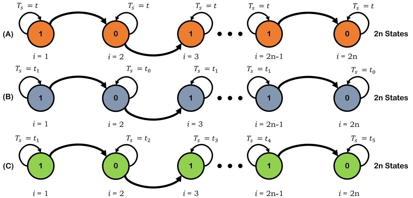
FIGURE 7. A diagram of possible transmissions that can create leftover chemicals ( \theta_{ISI} ). In each sub-plot the bits are shown as circle diagrams and their duration is defined as T_s . In this model, shown in Section III, the bits are defined as the continuation of the \theta function. For example, a transmission of 111 will have absorbed mass values of \theta_1(x, T) , \theta_1(x, 2T) and \theta_1(x, 3T) , respectively. Based on this behavior, each different bit is defined as a state ( i ) and can be seen in the sub-plots. (A) A sequential transmission of 1's and 0's continuously (i.e., 110011001100...) (B) A transmission of uneven amounts of 1's and 0's (i.e., 100010001001...) (C) A transmission where the transmission ends with chemical introduction into the environment (i.e., 101100011101111...).
