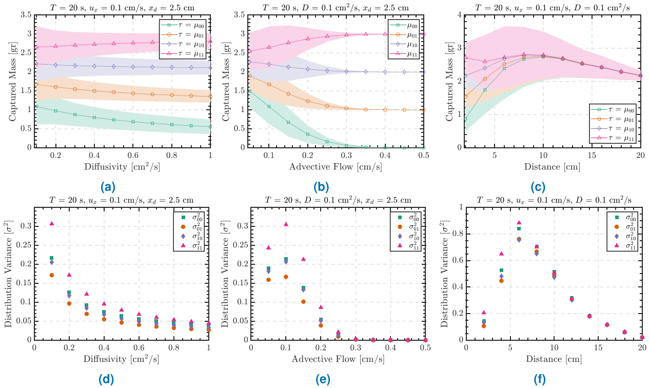
FIGURE 14. Simulation results of the symbol distribution of the transmitted symbol. In the plot \mu are the mean value of the received mass of their respective symbol (00, 01, 10, 11) (a), (b), (c) and the symbol variance (d), (e), (f) of the following parameters: Diffusivity (a), (d); Advective flow (b), (e); Transmission distance (c), (f).
