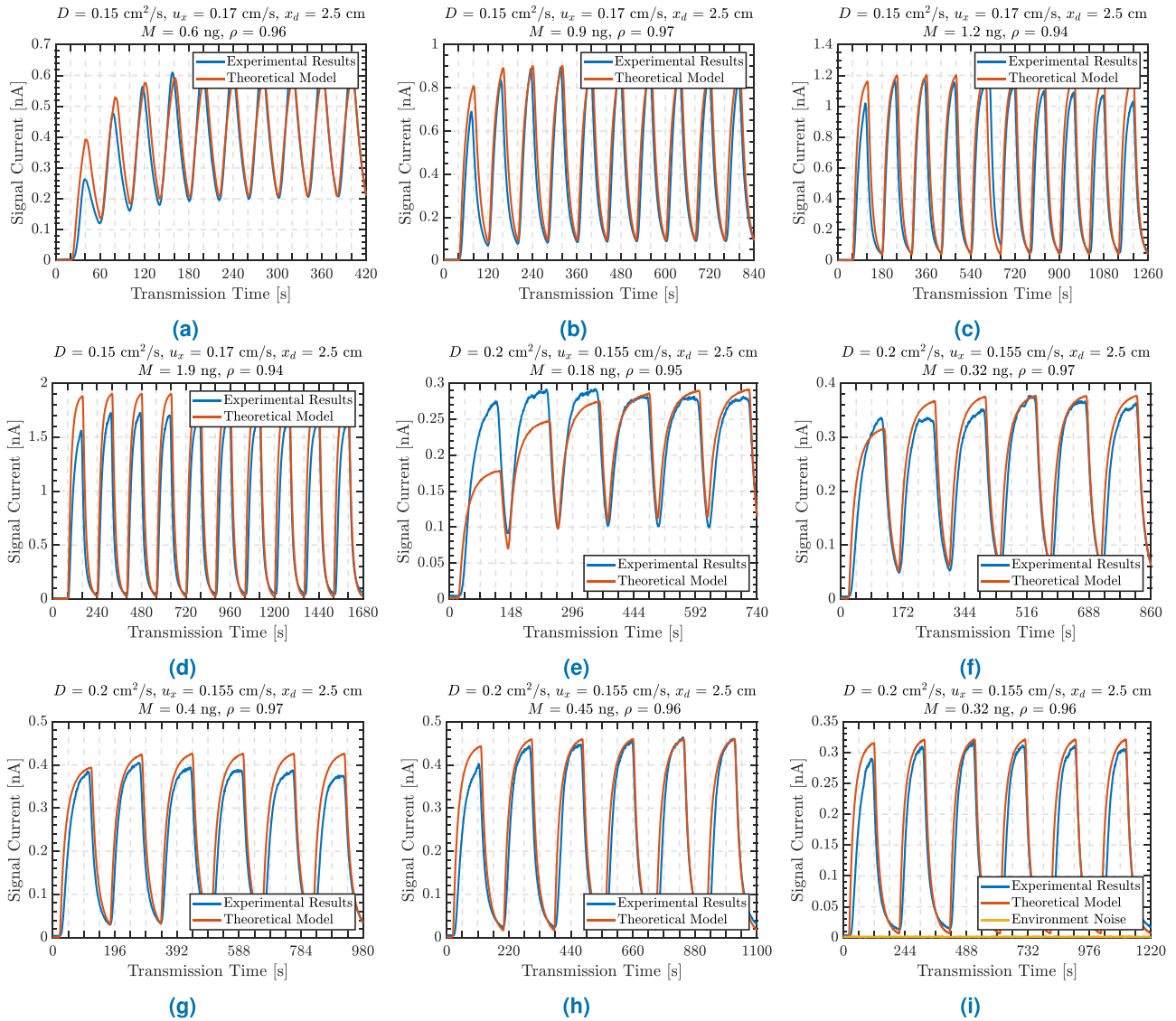
FIGURE 8. Results along with theoretical comparison of k (a-d) and one-to-zero (e-i) experiments (Noise Parameters: \mu_N = 1.21 \times 10^{-3} , \sigma_N = 3.098 \times 10^{-4} ): (a) Bit transmission of 01 pairs (b) Bit transmission of 0011 pairs (c) Bit transmission of 000111 pairs (d) Bit transmission of 00001111 pairs (e) Bit transmission of 1111101111 pairs (f) Bit transmission of 11111001111 pairs (g) Bit transmission of 1111100011111 pairs (h) Bit transmission of 11111000011111 pairs (i) Bit transmission of 1111100000111111 pairs.
