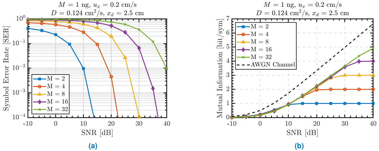
FIGURE 12. (a) Theoretical results of the Symbol-error rate of M-ary transmission (b) Theoretical results of the achievable information rate of M-ary transmission.
