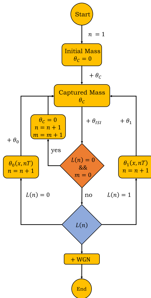
FIGURE 4. A diagram of the algorithm used in the simulation On-Off Keying (OOK) of macro-scale molecular communications.
