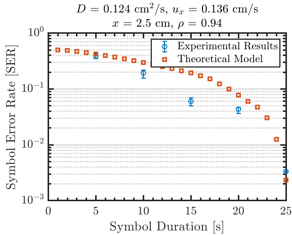
FIGURE 10. Experimental results of the symbol-error-rate (SER) and comparison to the theoretical model.
