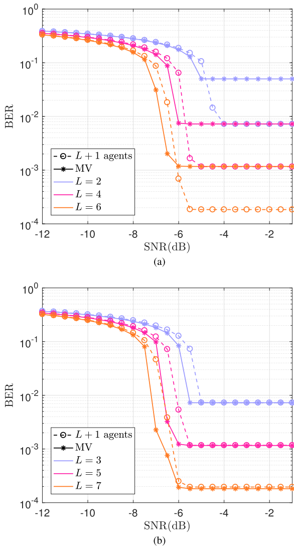
FIGURE 14. Comparison between one additional agent and a helper for more independent sources, where p_i = 0.05 . (a) L is even. (b) L is odd.
