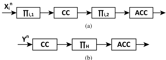
FIGURE 9. The structure of encoders. (a) Agent encoder i . (b) Helper encoder H .
