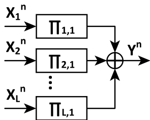
FIGURE 8. Generation of helper information by modulo-2 sum.
