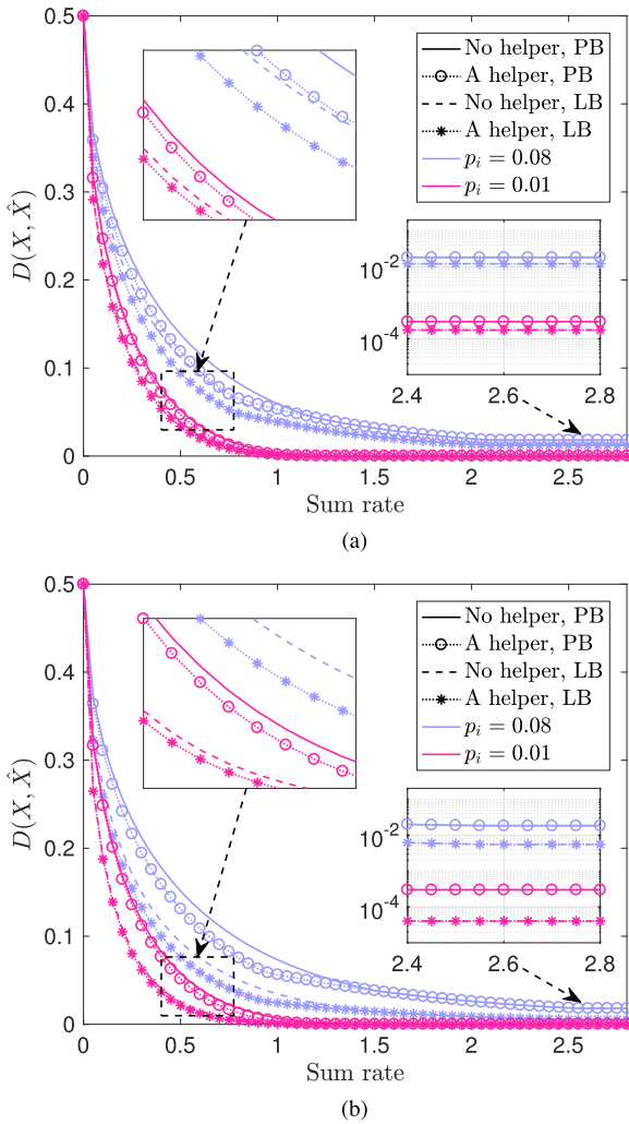
FIGURE 6. The trade-off of rate-distortion with diverse number of agents. (a) L = 3 . (b) L = 4 .
