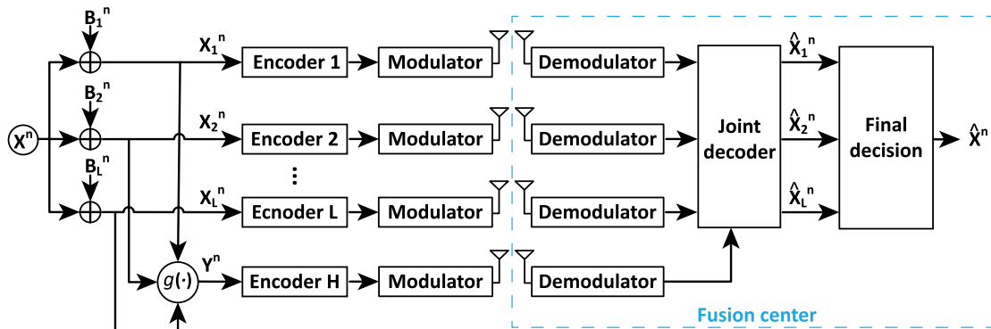
FIGURE 7. Simulation system.
