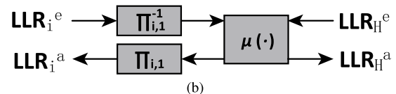
FIGURE 11. The structure of extrinsic information exchanger. (a) The helper information is generated by modulo-2 sum, where i, j \in \mathcal{L} and i \neq j . (b) The helper information is generated by majority voting.
