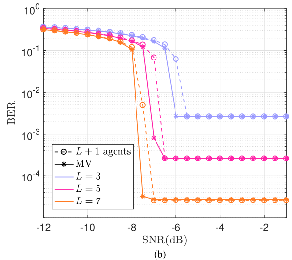
FIGURE 13. Comparison between one additional agent and a helper, where p_i = 0.03 . (a) L is even. (b) L is odd.
