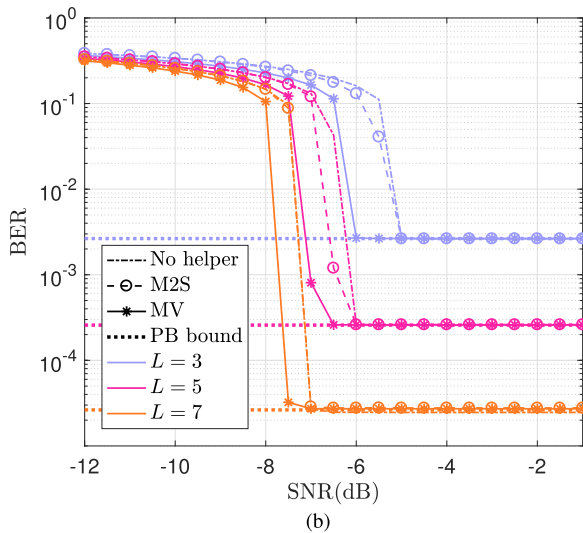
FIGURE 12. Comparison of simulation results between different structures of helper, where p_i = 0.03 . (a) L is even. (b) L is odd.
