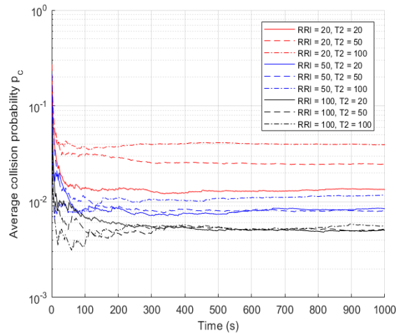
FIGURE 5. Average collision probability p_c with different combinations of RRI and T2.
