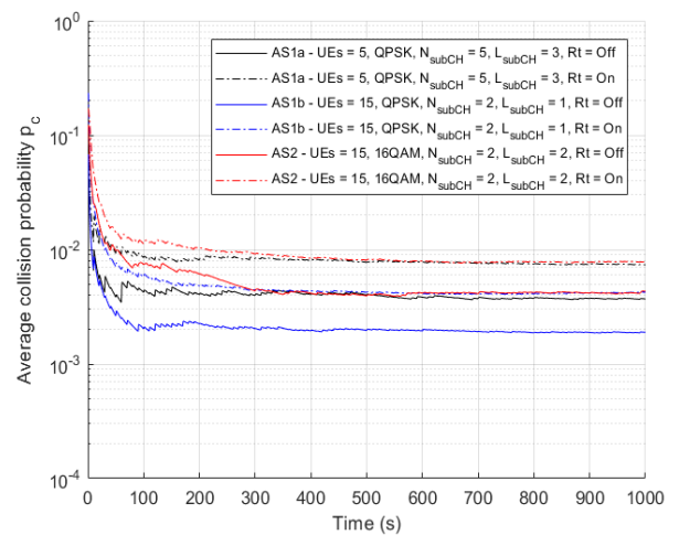
FIGURE 9. Average collision probability for different application scenarios (ASs).
