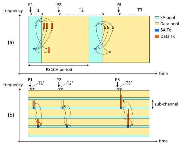
FIGURE 1. Resource allocation: a) modes 1 and 2, b) modes 3 and 4.
