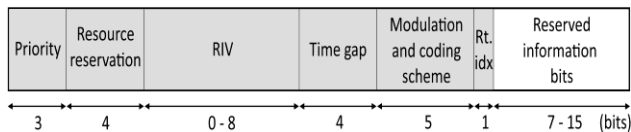
FIGURE 10. SCI format 1 fields.
