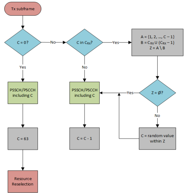
FIGURE 6. CLR scheduling mechanism for eV2X services.
