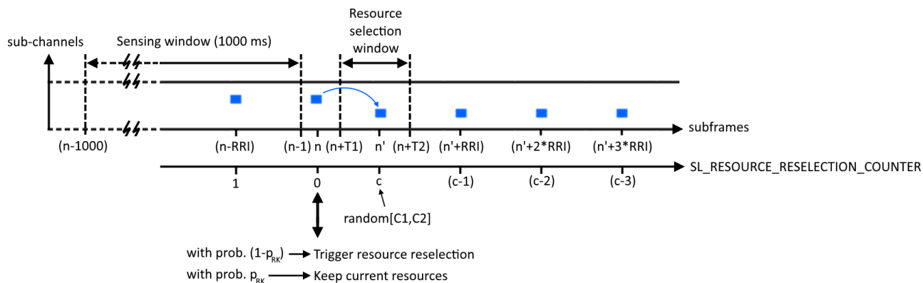
FIGURE 3. Resource reselection triggering in standardized sensing-based SPS procedure.
