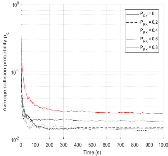
FIGURE 4. Average collision probability p_c with different reselection probability P_{RK} values.
