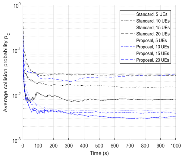
FIGURE 8. Average collision probability of the proposed CLR mechanism for different number of UEs in a dynamic scenario.
