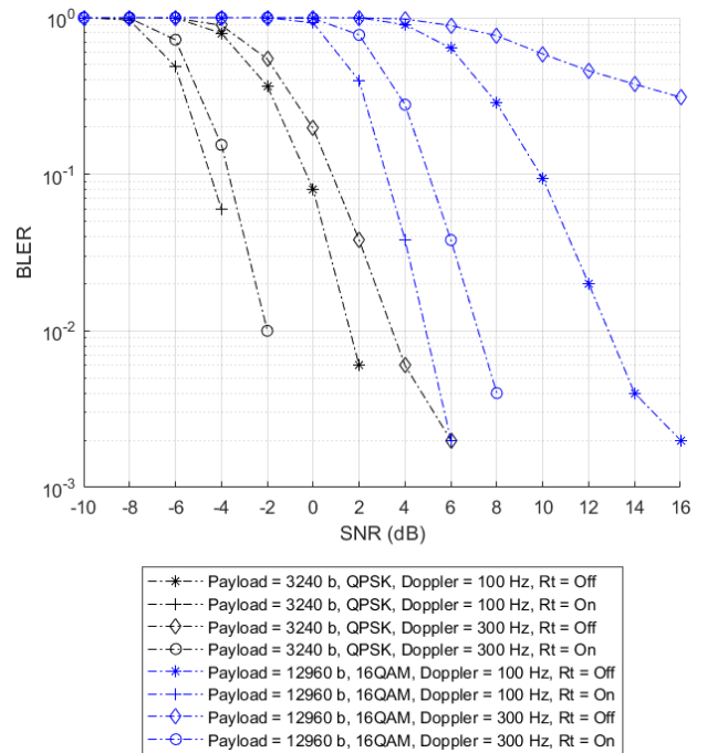
FIGURE 2. Achievable BLER vs SNR for different payload sizes, modulations, Doppler shifts and transmissions.
