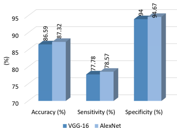
FIGURE 4. Percentage of Accuracy, sensitivity, and specificity of the system using VGG-16 and AlexNet.
