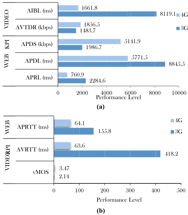
FIGURE 7. The average WEB and Video measured KPIs for 4G and 3G technologies. (a) The AIBL, AVTDR, APDS, APDL and APRL. (b) The average APRTT, AVRRTT and vMOS.
