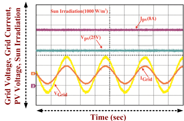
FIGURE 8. Experimental steady state PV responses with grid.
