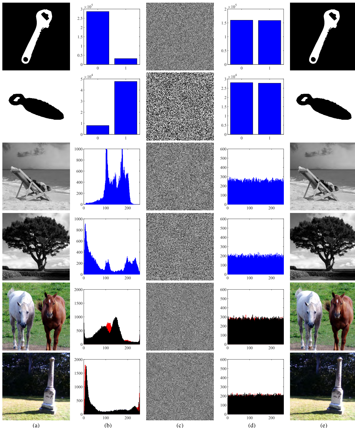
FIGURE 8. The experiment results of IES-JPDF. (a) The plain-images including binary, grayscale and color images; (b) The histograms of (a); (c) The cipher-images; (d) The histograms of (c); (e) The decrypted images.
