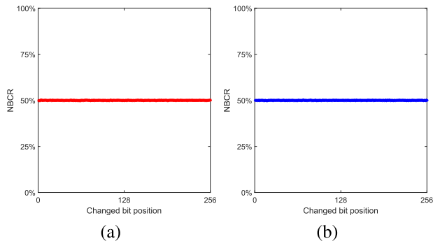
FIGURE 11. The key sensitivity analysis results. (a) The NBCR between two cipher-images encrypted from an identical image with two secret keys owning one bit difference, (b) NBCR between two decrypted images from an identical cipher-image with two secret keys owning one bit difference.
