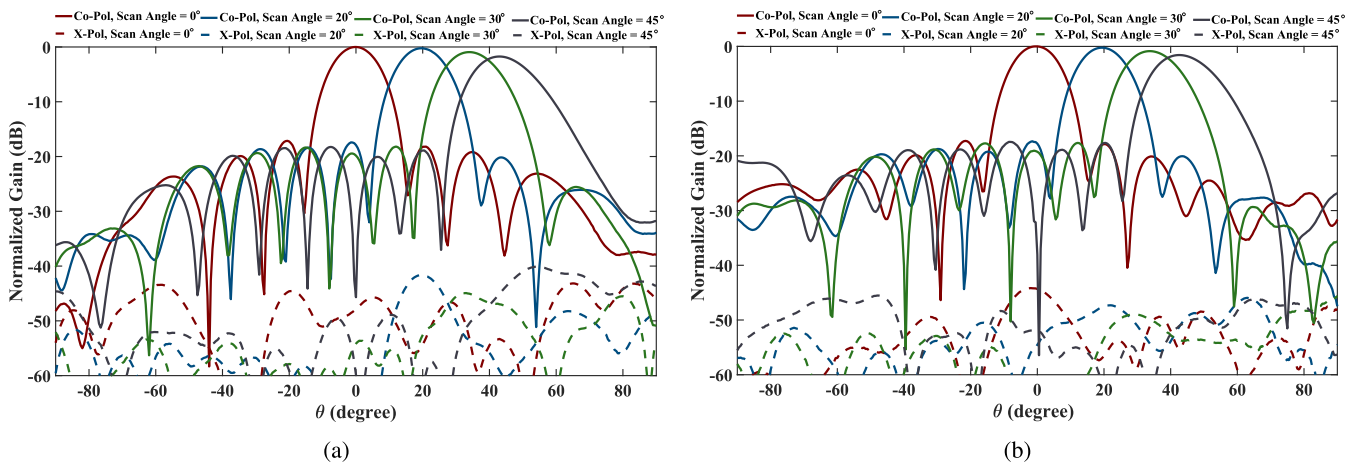
FIGURE 10. Measured scan radiation pattern of the central 2 × 8-element array in the fabricated 4 × 10-element array at 2.7 GHz, 2.8 GHz, and 2.9 GHz; (a) H-pol, \varphi = 0^\circ ; (b) H-pol, \varphi = 90^\circ .
