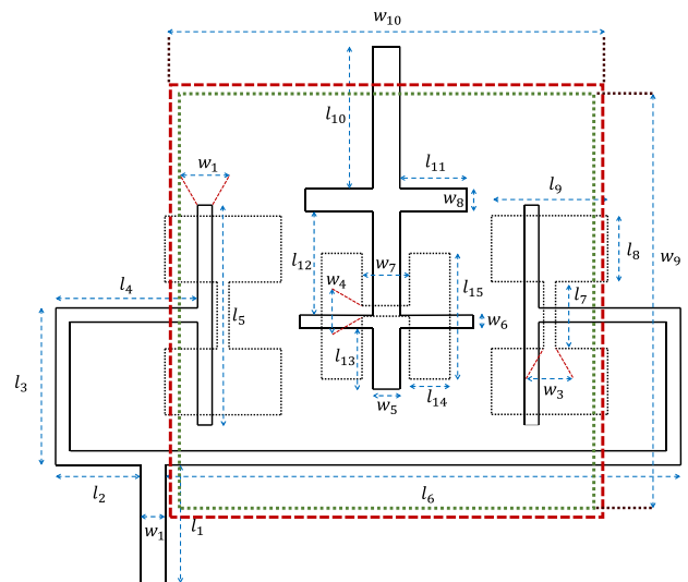
FIGURE 2. Parameters of the proposed antenna.
