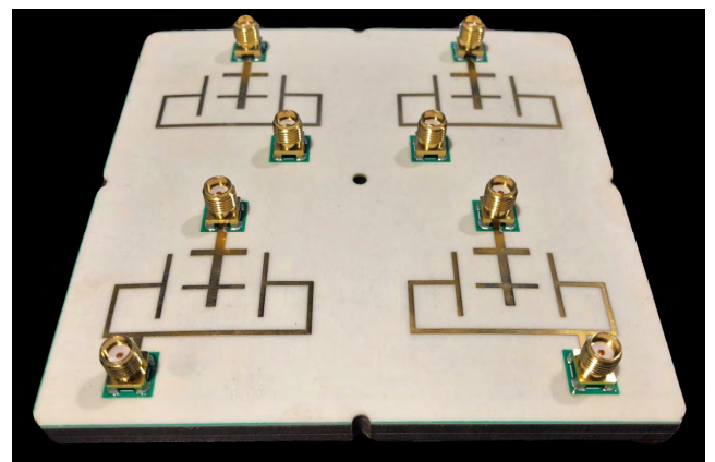
FIGURE 7. Fabricated 2 \times 2 -element subarray.
