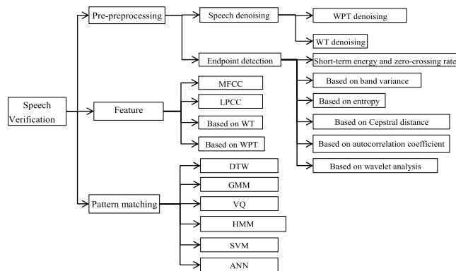
FIGURE 1. Taxonomy of speech verification.
