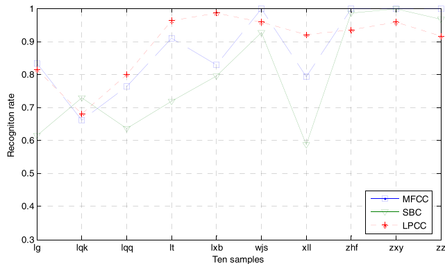
FIGURE 10. Performance comparison of MFCC, LPC and SBC in the second group.
