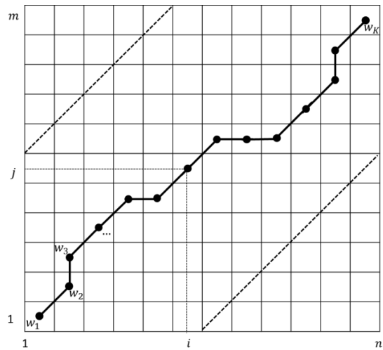
FIGURE 3. An example warping path.
